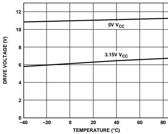
Figure 8. Drive Voltage ( V_{GATE} - V_{CC} ) vs. Temperature
