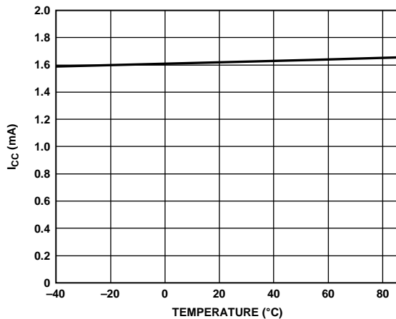
Figure 7. Supply Current vs. Temperature (Gate On)
